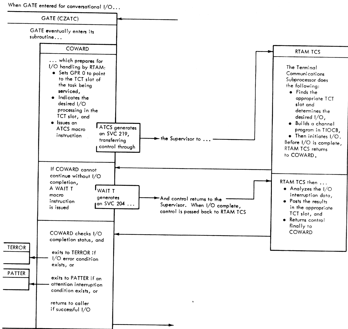
Figure 7. Interaction of COWARD and RTAM TCS
