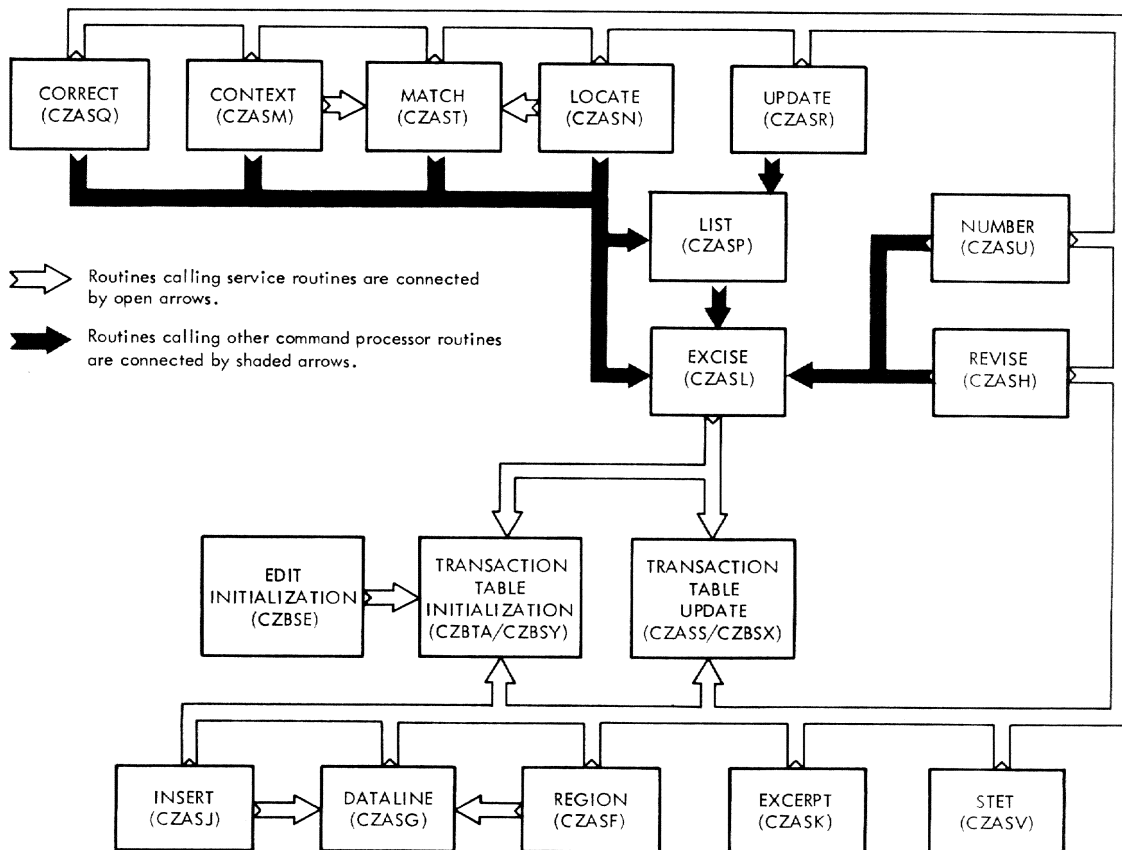
Figure 9. Interrelation of Text Editor Command Processor and Service routines
