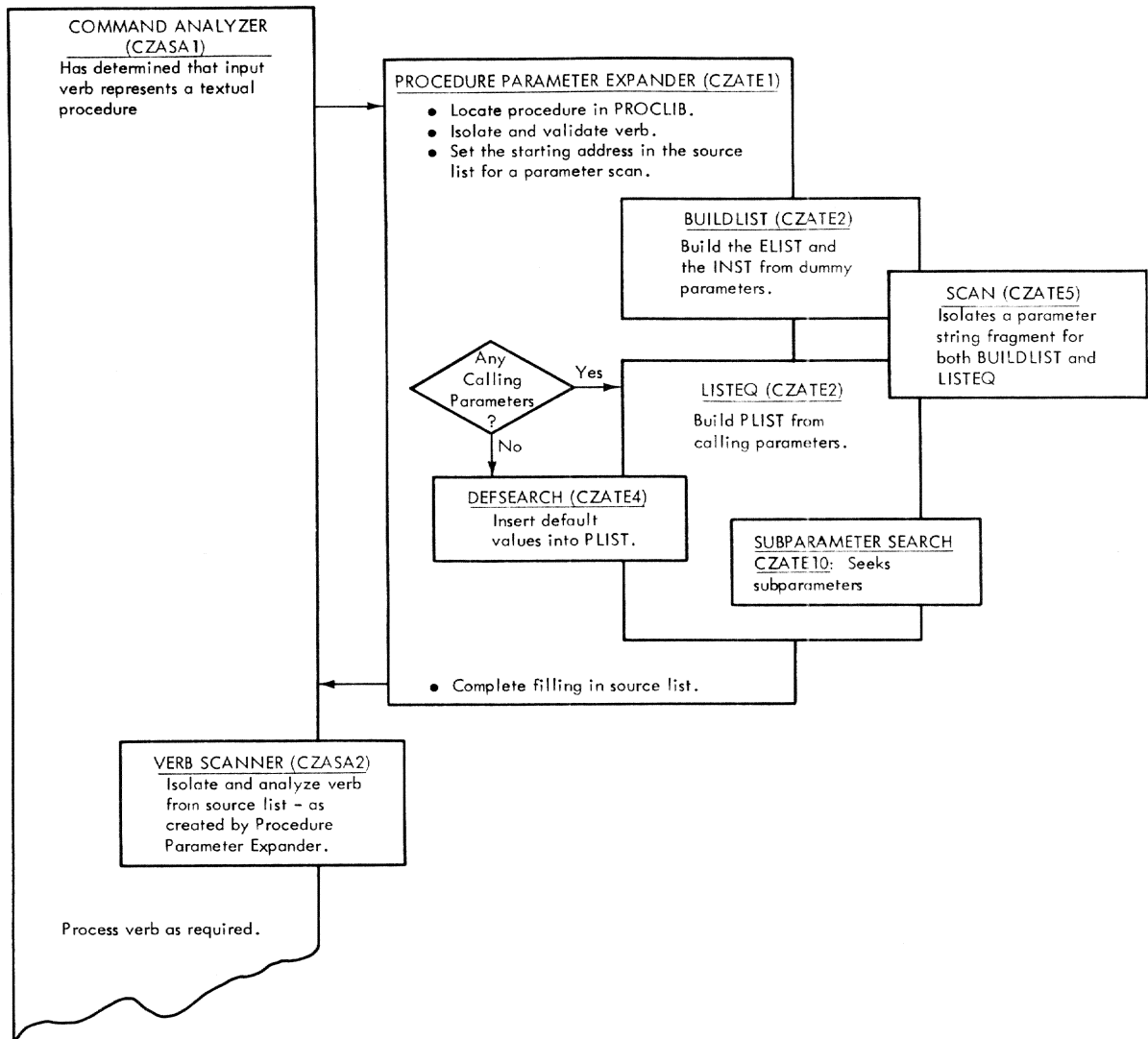
Figure 4. Execution of a textual procedure
