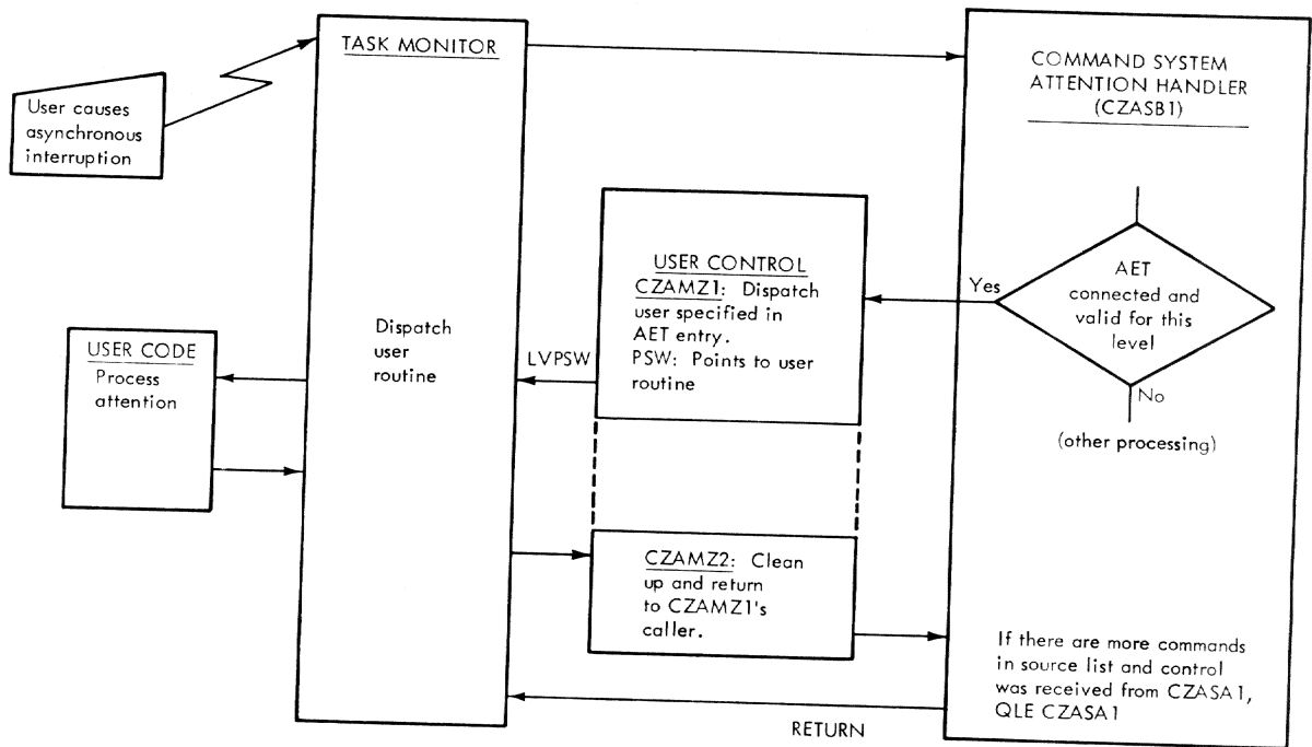
Figure 8. Attention processing with AET connected
