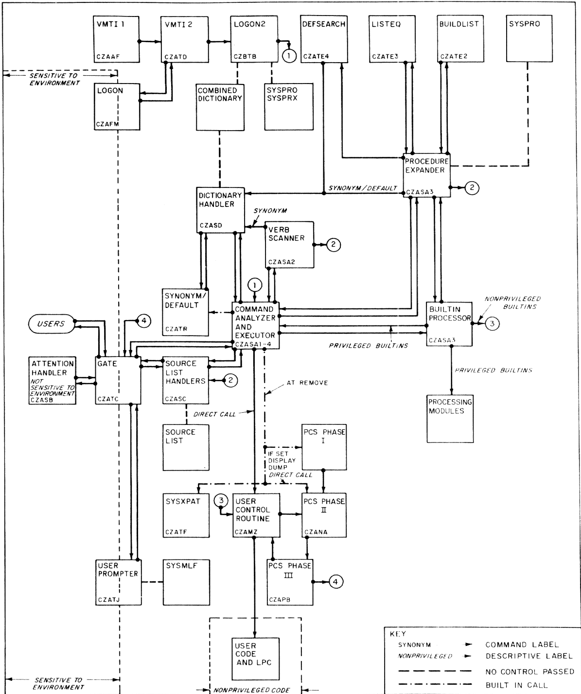
Figure 6. Modular relationship of the command system
